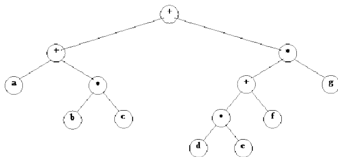
Inorder traversal yields: a + b * c + d * e + f * g
